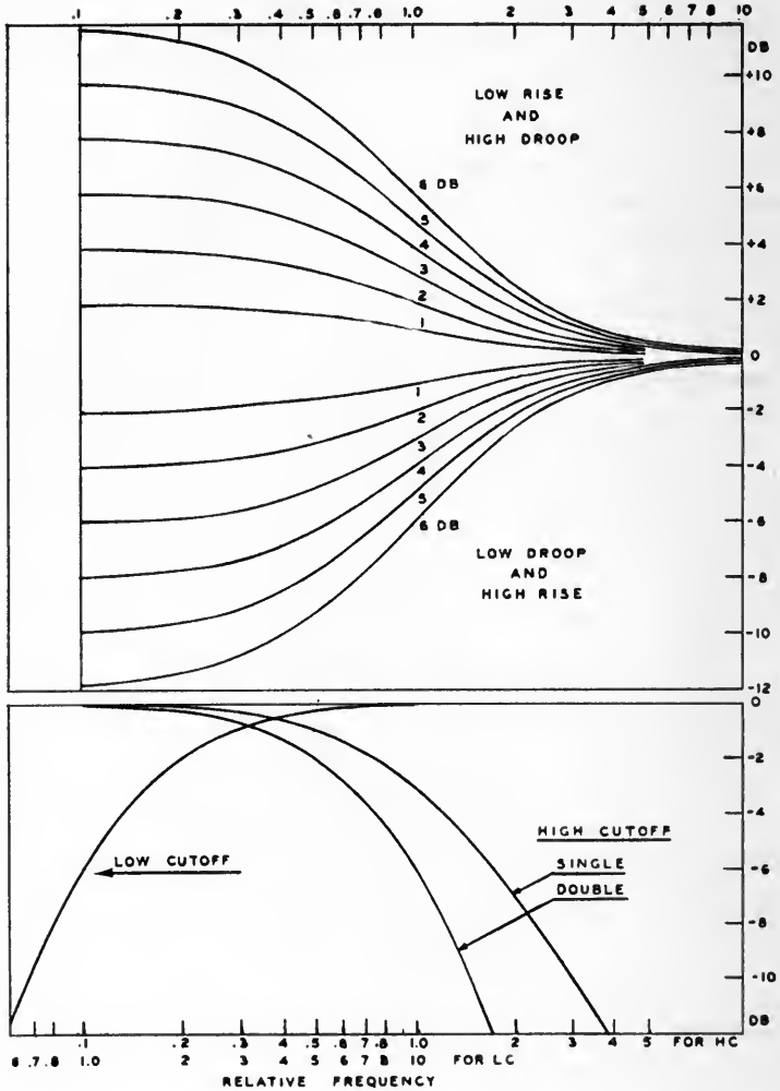
FIG. 1. Generalized relative response of equalizer sections which raise or depress one end of the spectrum.
